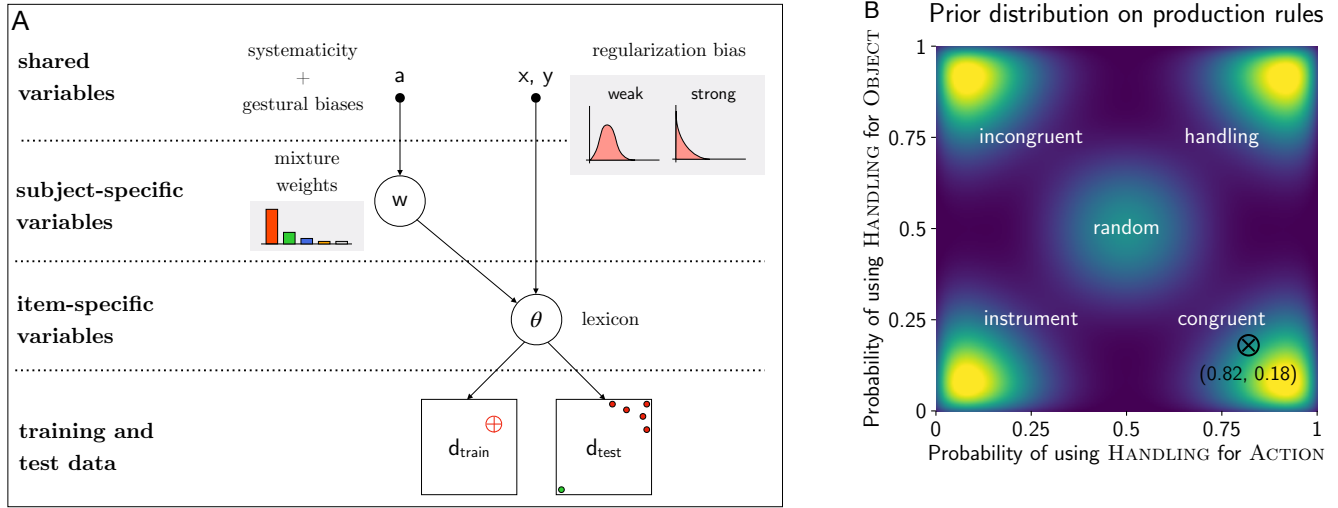
Figure 3: A. The hierarchical Bayesian model and its various levels of shared and independent structure. Two model variations are derived from the full model depicted here: In the no item-specific inferences model, the lexicon \theta is no longer item-specific and thus moved up next to the mixture weights w . In the no language-wide inferences model, the mixture weights w node is shared across all subjects instead of subject-specific and thus moved up next to parameters a , x and y . B. The hypothesis space for a single production rule \theta of the lexicon. Here we depict a prior distribution over \theta with equal mixture weights w = (0.2, 0.2, 0.2, 0.2, 0.2) and with regularization strengths x = 11, y = 2 and random component r = 8 . Brighter colors correspond to higher probability regions.
